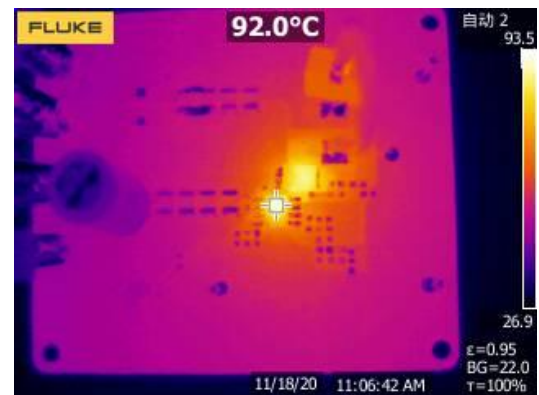
Figure 24. Thermal, 24VIN, 3.3Vout, 5A
