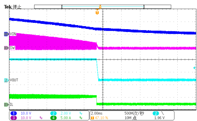
Figure 14. Power down(Iload=3.5A)
