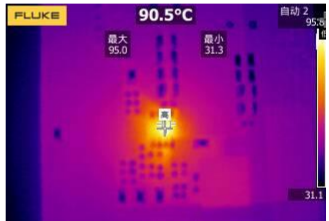
Figure 25. Thermal, 3.3Vout/3.5A
