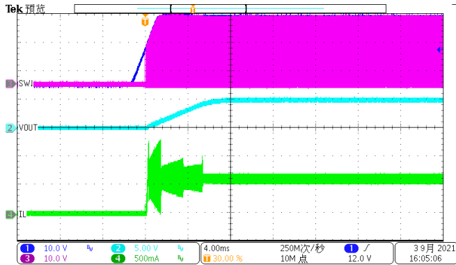
Figure 11. Power up(Iload=0.6A)
