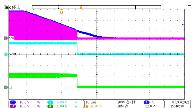
Figure 12. Power down(Iload=1A)
