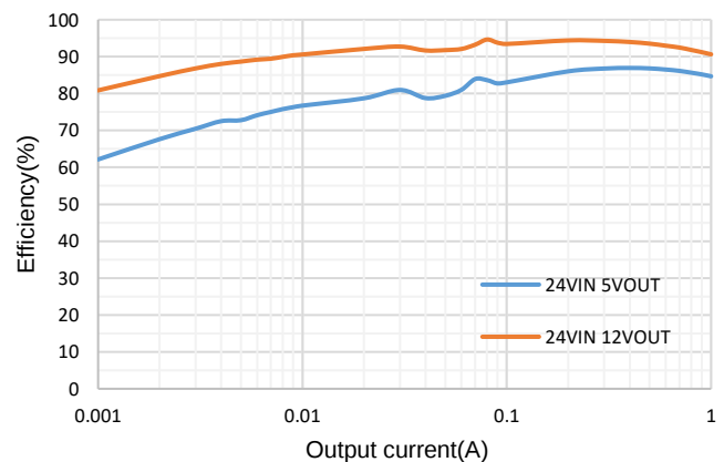
Efficiency, Vin=24V
