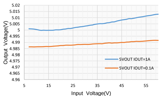
Figure 6. Line Regulation
